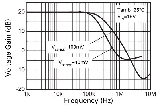
Frequency Response
