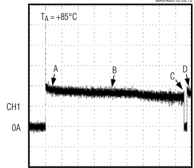
SHORT-CIRCUIT RESPONSE ( V_{BIAS} = 40\text{V} )
