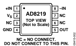
Figure 2. Pin Configuration
