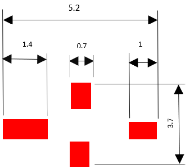
PCB Footprint
