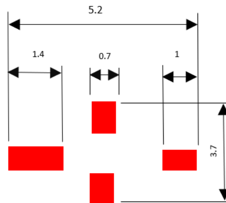
PCB Footprint
