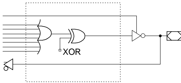
Combinatorial I/O Configuration for Complex Mode
