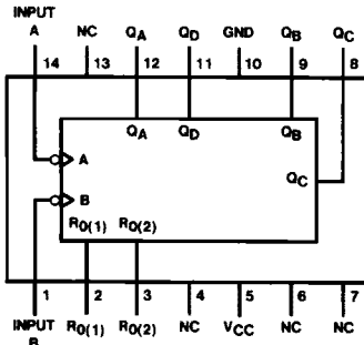
Dual-In-Line Package
