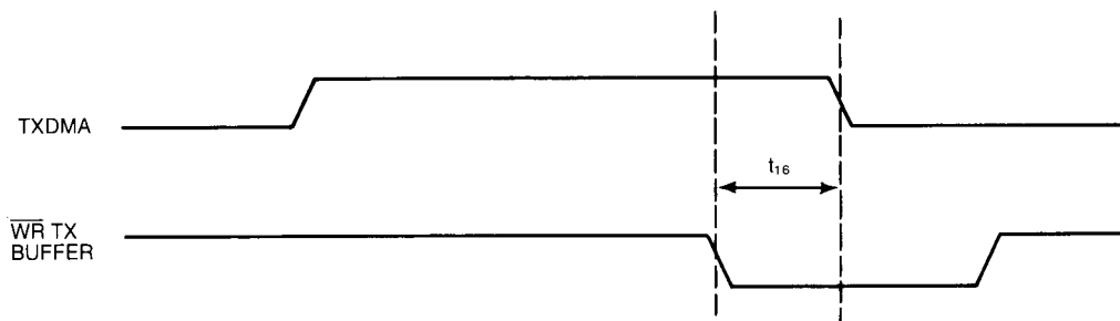
Fig. 8—TX DMA ACKNOWLEDGE TIMING
