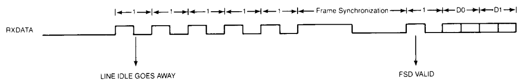
Fig. 16—COM52C50 RECEIVE START TIMING
