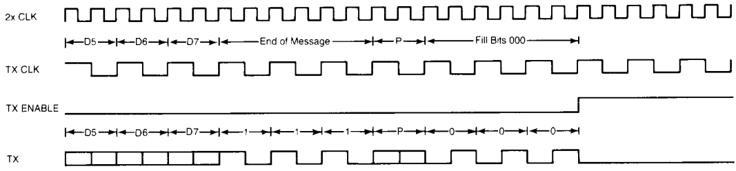
Fig. 15—COM52C50 TRANSMIT END TIMING
