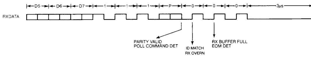
Fig. 17—COM52C50 RECEIVE END TIMING
