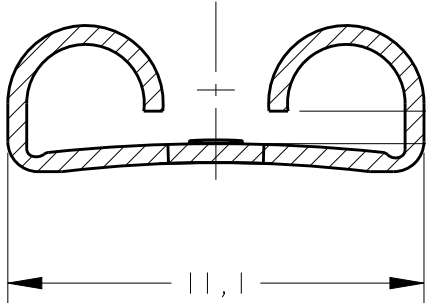
SECTION B - B SCALE 5:1
