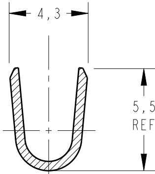
SECTION C - C SCALE 5:1
