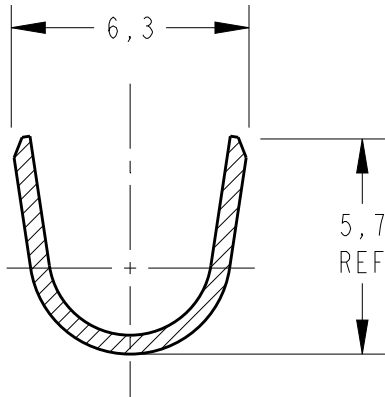
SECTION D - D SCALE 5:1
