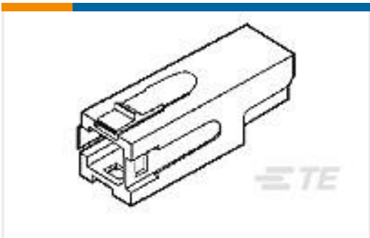
TE Part #53884-1 HSG ASSY,PWR LK,SRS2,1 POS,BLU
