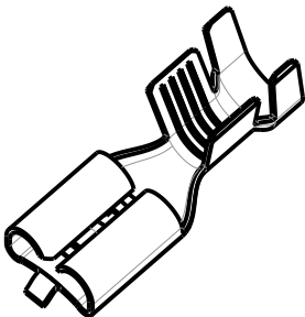
PERSPECTIVE VIEW SCALE 2:1
