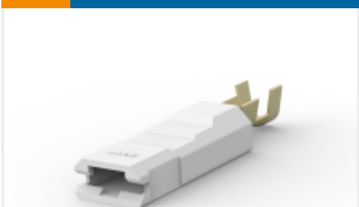
TE Part #520963-1 ULTRA POD: Straight, Receptacle Assembly, Unplated, .250 inch
