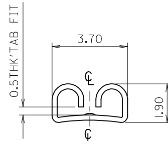
VIEW "A"
