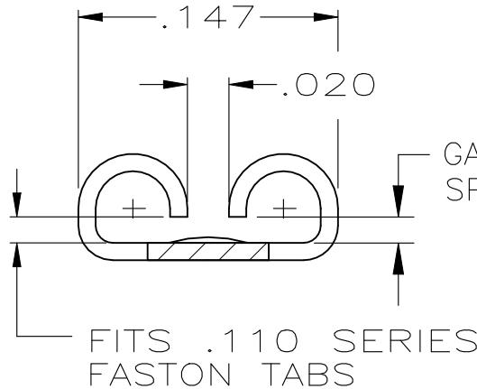
VIEW Z-Z SCALE 10:1
