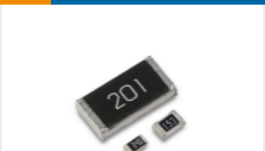
TE Part #2176326-9 CRGP 0603 47R 1%
