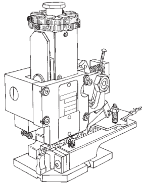
Heavy Duty Miniature Quick-Change (End-Feed Type Applicator)
