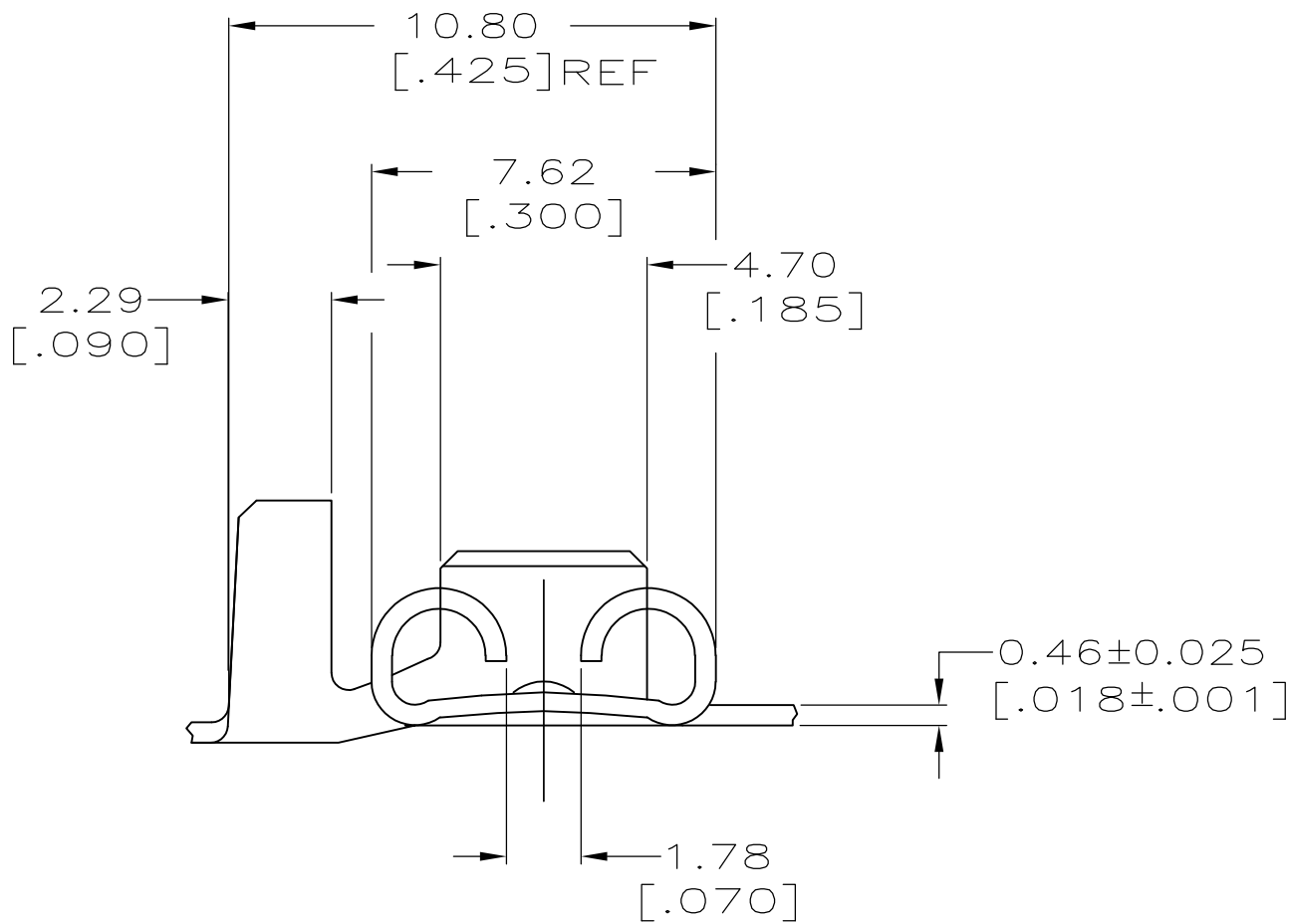
SECTION B-B
