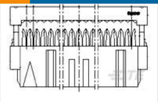
TE Part #3-215915-4 AMP-LATCH 15.2 HIGH TAPE
