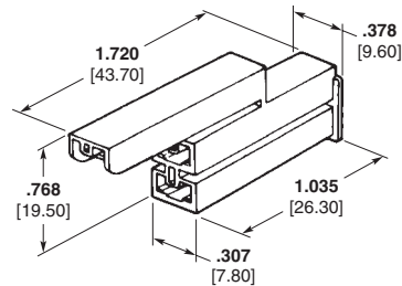
A — 3 Circuit For Micro-Switch
