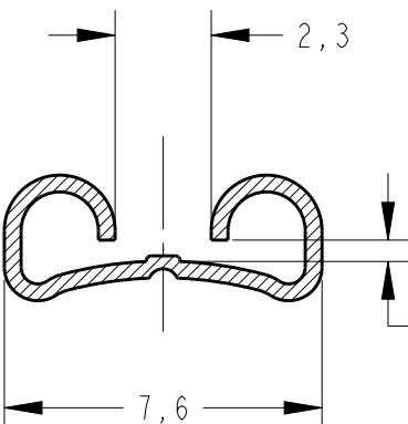
SECTION X - X SCALE 5:1
