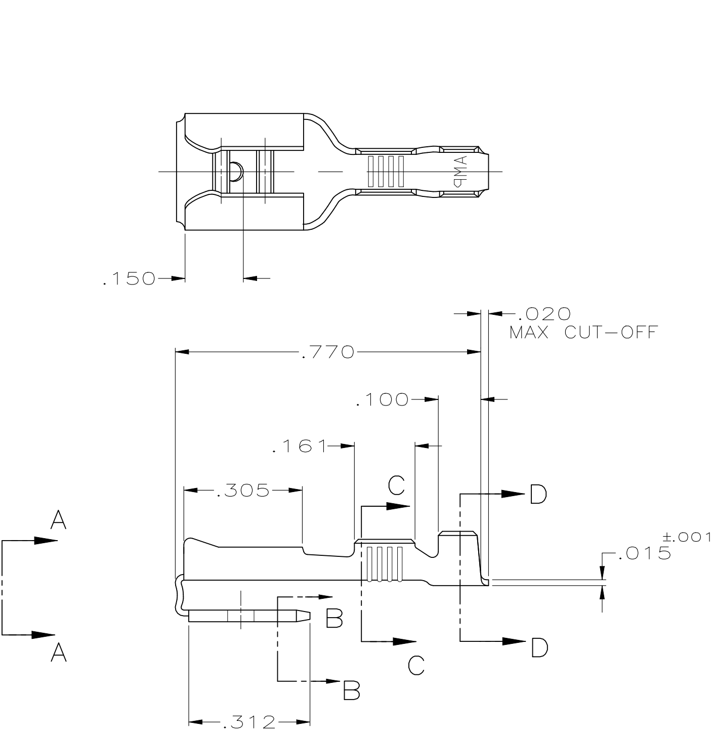
— FITS .250 SERIES FASTON TAB VIEW A—A SCALE 8:1
