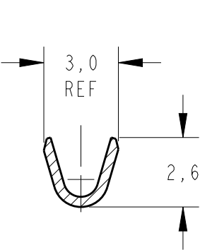
SECTION B-B SCALE 5:1
