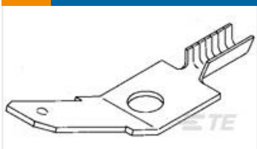
TE Part #63136-1 250 AMVAR TAB 200-860 TPBR
