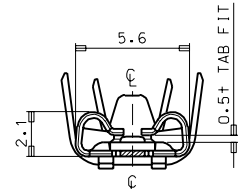
VIEW "A"
