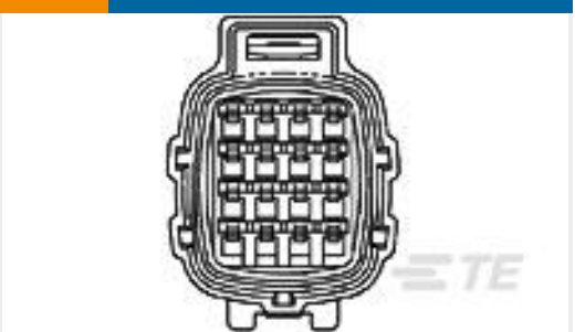
TE Part #368047-1 E-S MK-2(+) 16P PLUG ASSY
