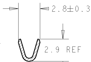
SECTION C-C SCALE 4:1
