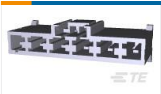
TE Part #4-178841-2 AMP U/P SGL ROW HDR ASSY V 6P
