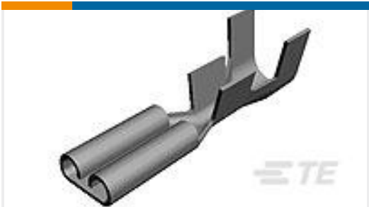
TE Part #42219-1 250 FASTON REC 18-14 AWG NPST
