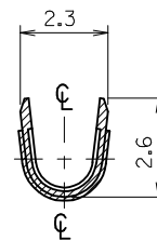
SECTION:C-C"
