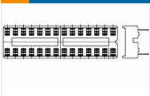
TE Part #1-2199298-4 16P,DIP SKT,300 CL,LDR,PB FREE
