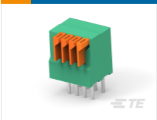
TE Part #1-2834015-4 4POS 2.54MM TES CONN.
