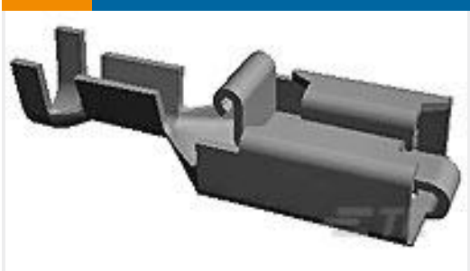
TE Part #154717-1 PL 250 REC TERMINAL 13-11 AWG BR
