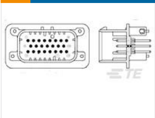
TE Part #776262-1 14POS,PIN DIA 1.3,HDR ASSY, 180DEG,COD 1
