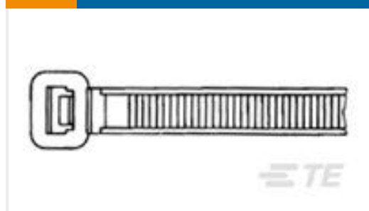
TE Part #2-160967-2 CABLE TY 98X2.5 BLA
