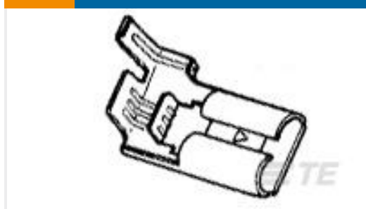
TE Part #1-1627087-0 RECEPTACLE, FLAG QC 4.8x0.8 (H25411)
