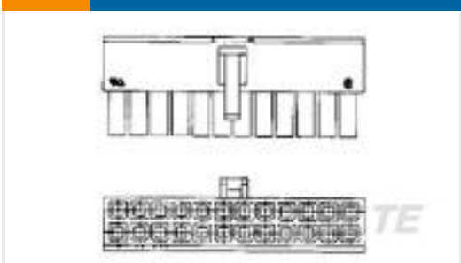
TE Part #1586765-6 6P RCPT VAL-U-LOK GW
