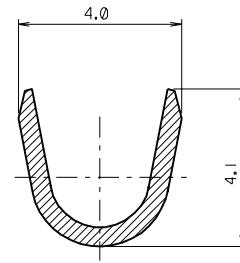
SECTION:D-D*
