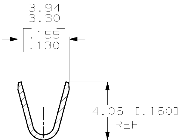
SECTION B-B SCALE 6:1
