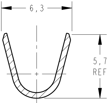
SECTION D-D SCALE 5:1
