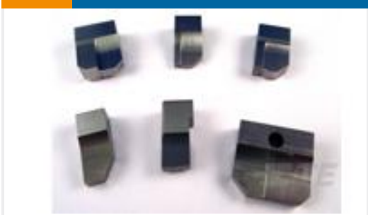
TE Part #1-690618-9 ANVIL SPLICE TYPE
