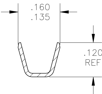
SECTION Y-Y
