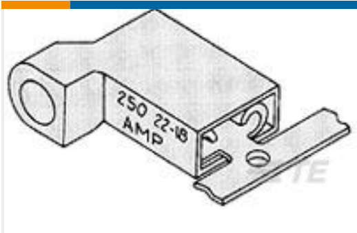
TE Part #9-520334-2 ULTRA-FAST 187 ASY REC 22-18 AWG TPBR
