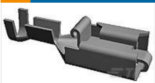
TE Part #880646-5 PL REC 0.5-1.0 MM2 0.40 X 52.32 PTPBR
