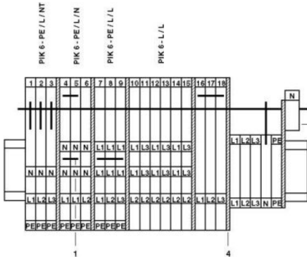
Circuit diagram
