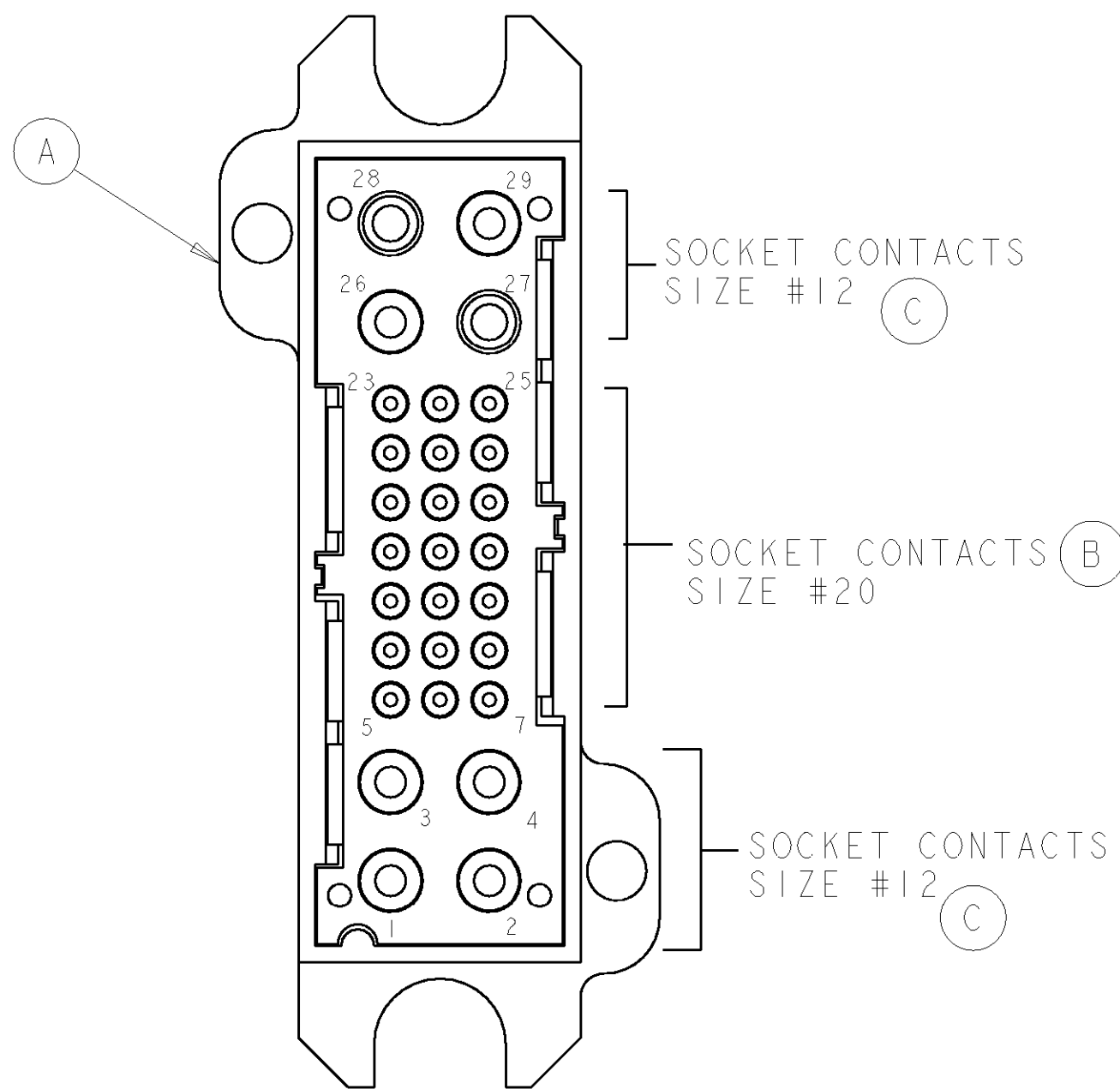
REAR VIEW
