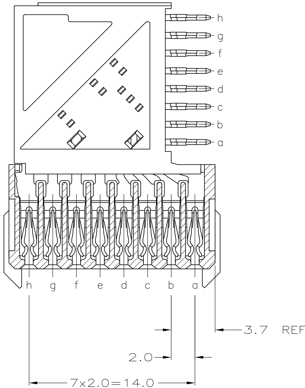
SECTION W-W
