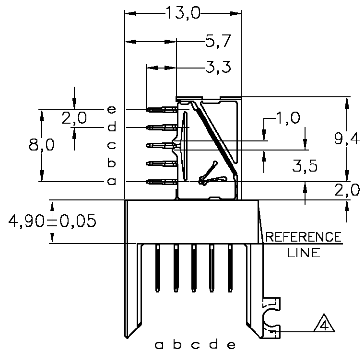
CONNECTOR ASSEMBLY EXEMPLARY LOADED
