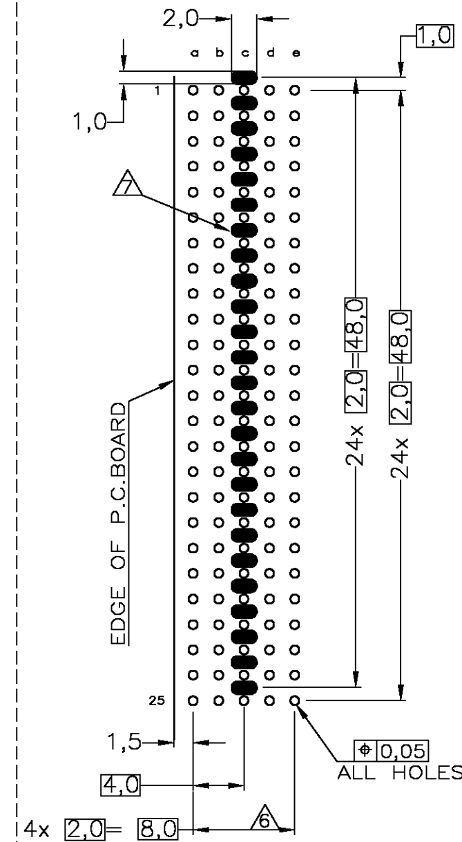
RECOMMENDED PCB-HOLE LAY-OUT COMPONENT SIDE SHOWN
