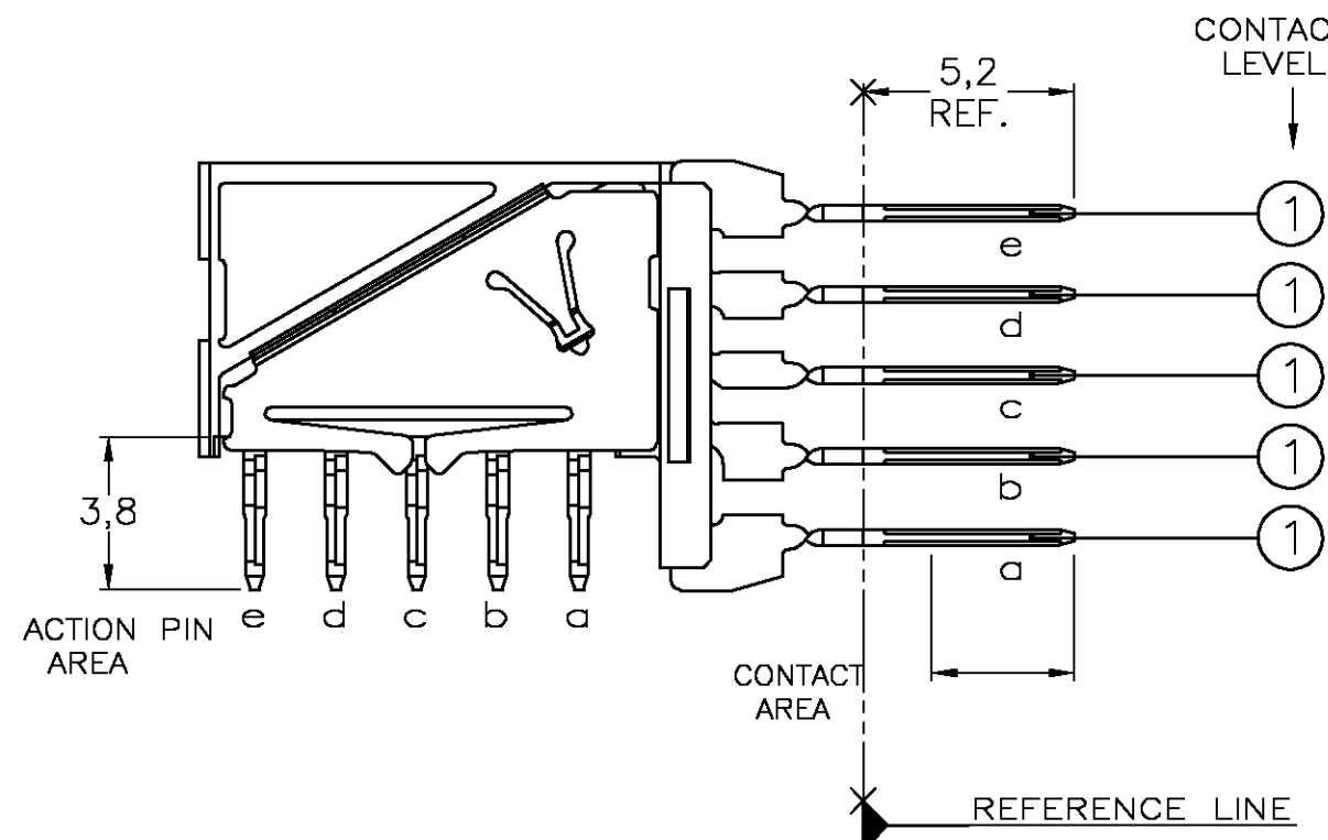
CONTACT DIMENSIONS
