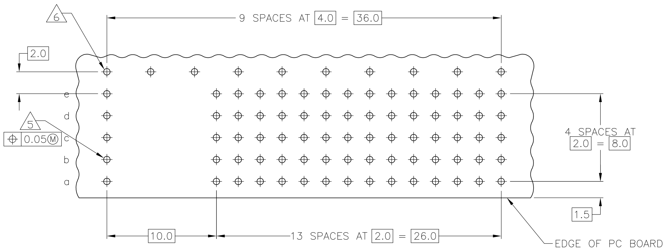
RECOMMENDED PC BOARD LAYOUT COMPONENT SIDE
