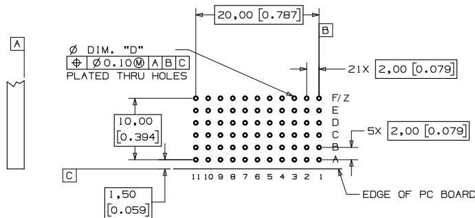
Recommended Hole Pattern for UHM-S055CL3-5AP1-XXXXX and UHM-S055CR3-5AP1-XXXXX
