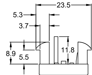
REAR COVER DETAIL
