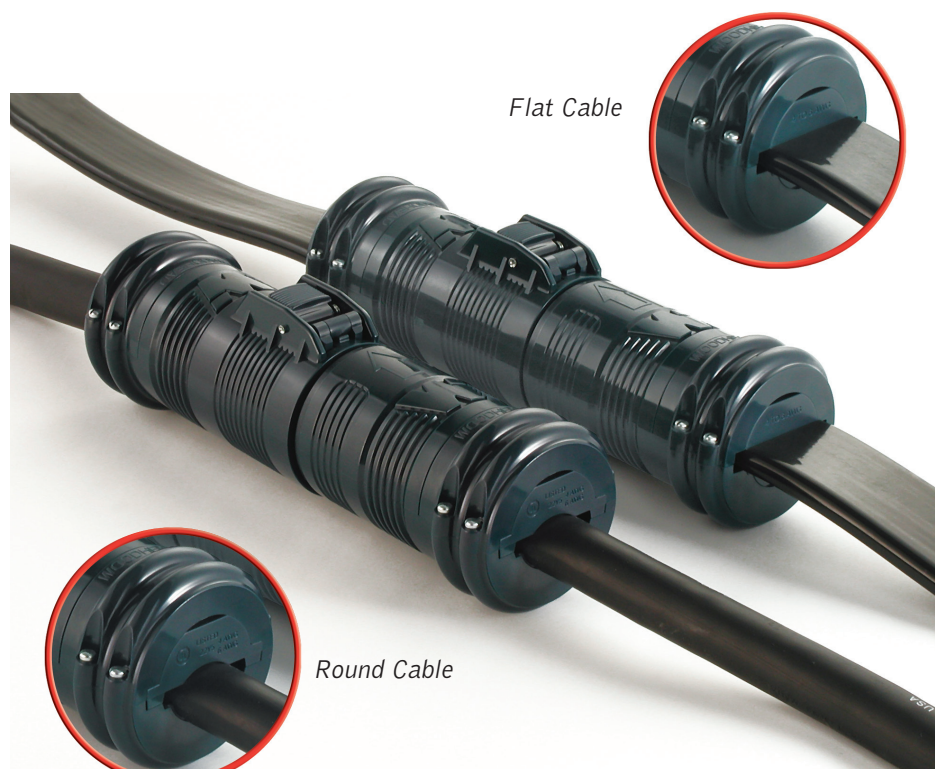
130150-0284 (Y560PF) Plug and 130150-0282 (Y560CF) Connector Shown
